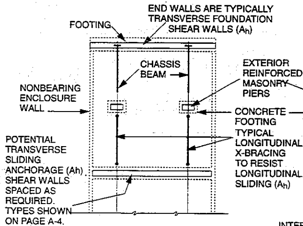
FOUNDATION PLAN
