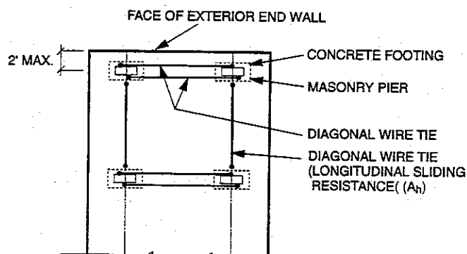
FOUNDATION PLAN
