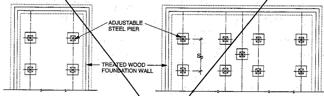
FOUNDATION PLAN
