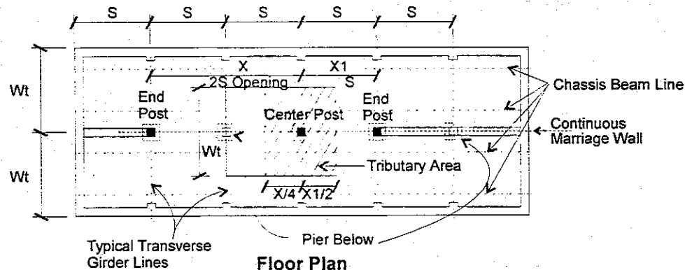
Floor Plan
