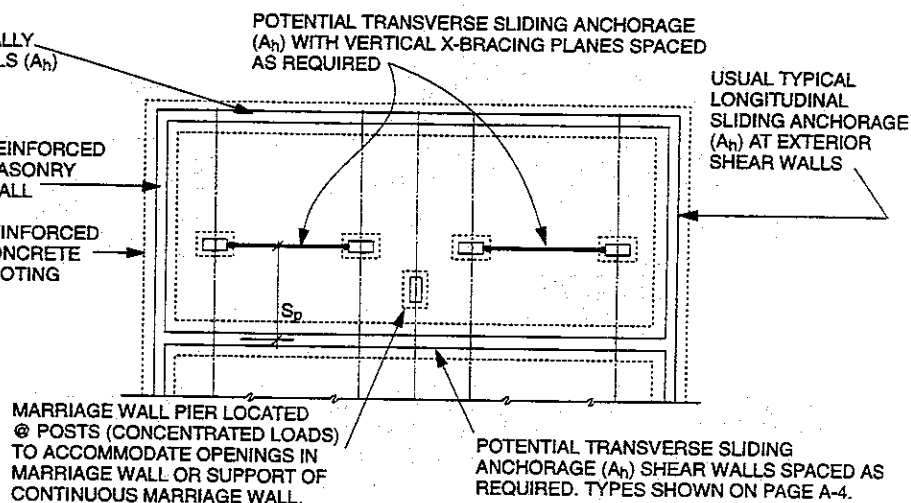
FOUNDATION PLAN
