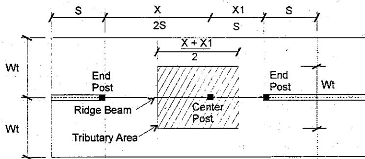
Roof Plan
