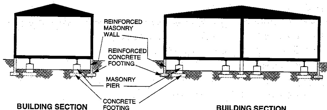
BUILDING SECTION
