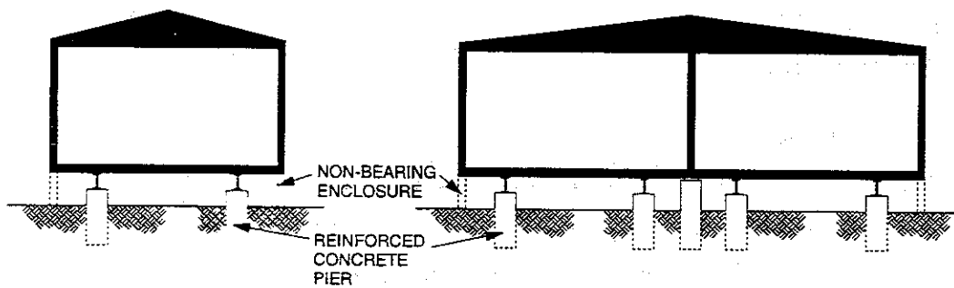
BUILDING SECTION
