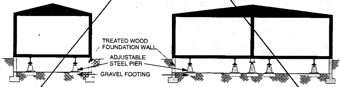
BUILDING SECTION
