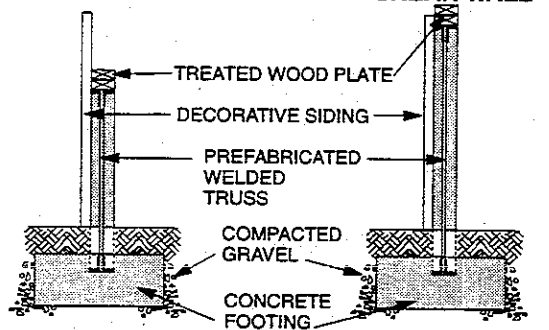
ALTERNATE TRANSVERSE END FOUNDATION SHEAR WALL
