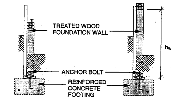
END TRANSVERSE FOUNDATION SHEAR WALL
