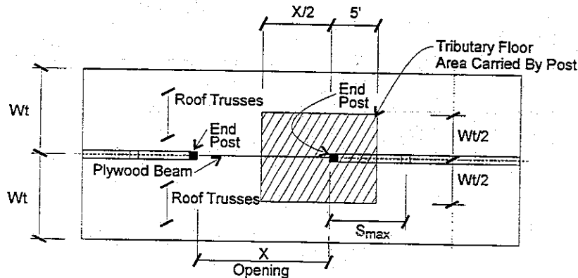
Roof Plan
