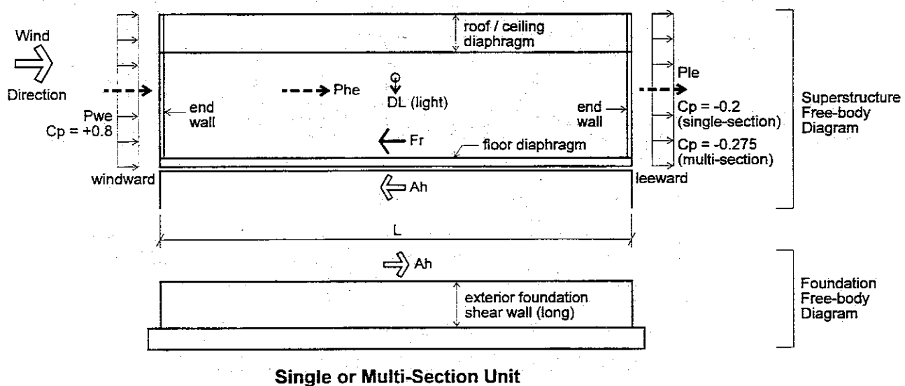
Wind Related Sliding - Longitudinal Direction
