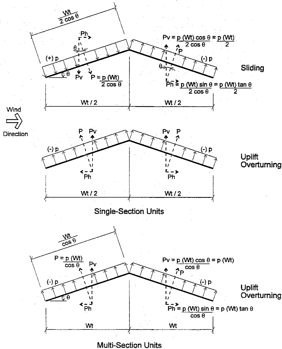
Roof Plane - Wind Components - Transverse Direction
